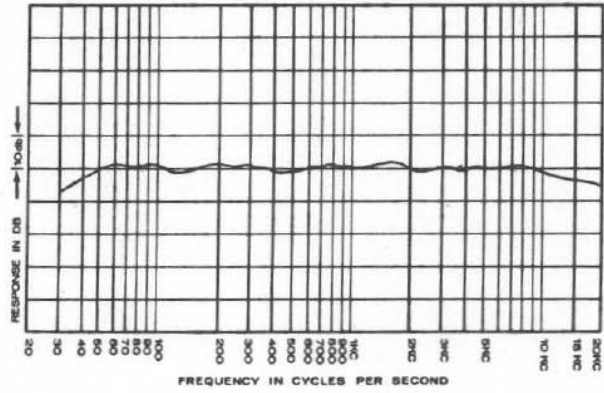
Figure 1 - Frequency Response
